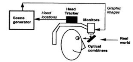
Figure 3: Optical See-Through Scheme.
